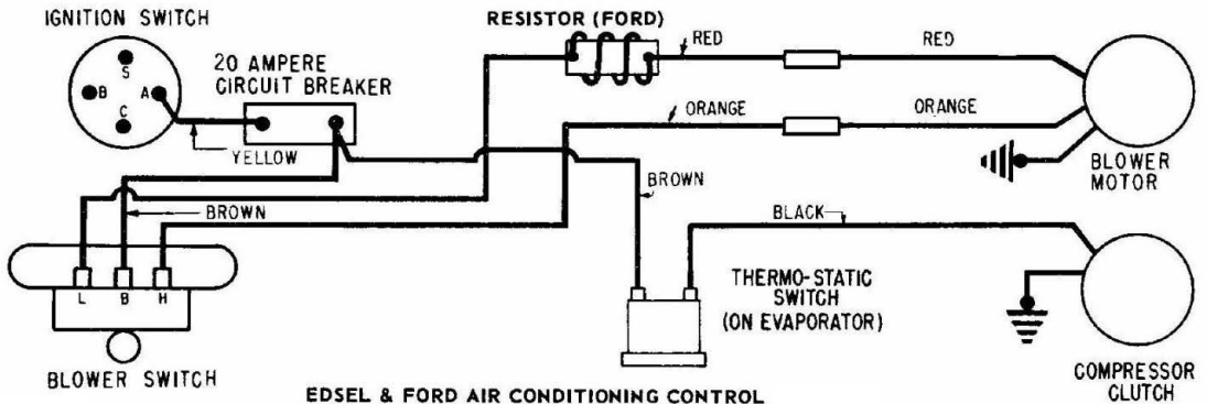
EDSEL & FORD AIR CONDITIONING CONTROL
