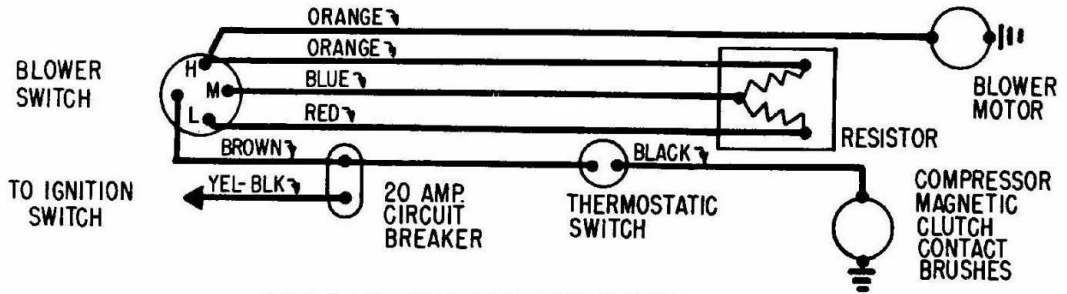
EDSEL & FORD AIR CONDITIONING CONTROL
